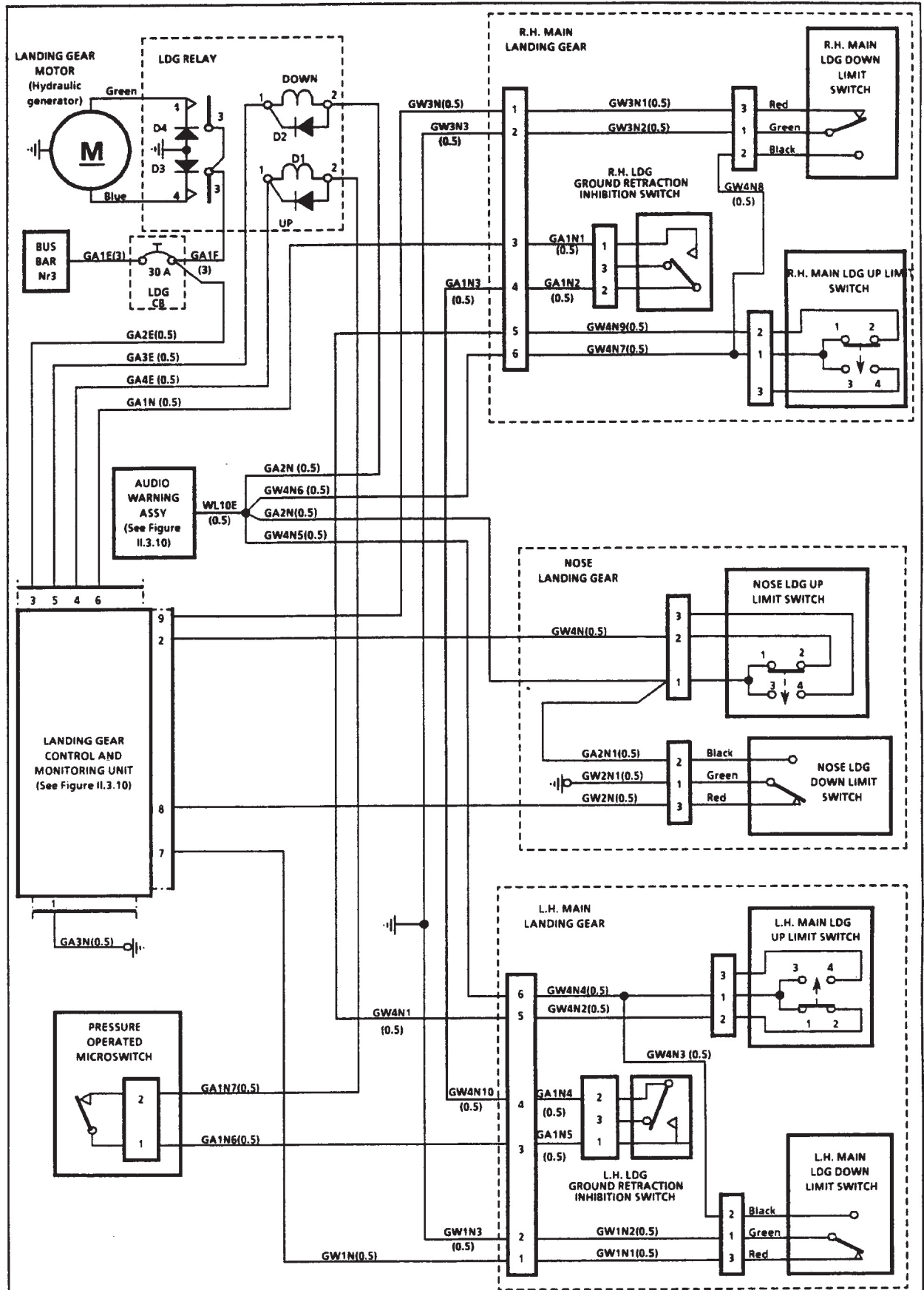
Figure II.3.11 - MICRO-CONTACTS TRAINS (avion au sol, trains sortis) LDG MICROSWITCHES (airplane on ground, LDG extended)
