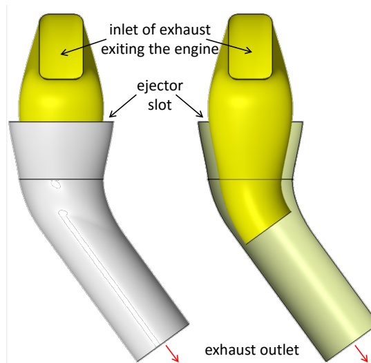
Fig. 4. The "FINAL-DESIGN" variant of the exhaust system
