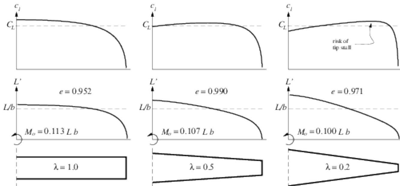
Figure 1: Load distributions, root bending moment, and span efficiency for three taper ratios. All three cases have AR=10 , and no wing twist.
