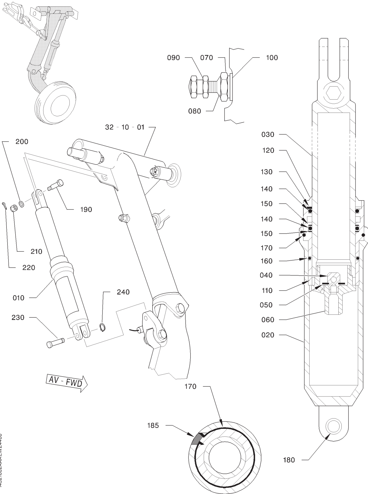
SHOCK ABSORBER FIGURE 1A
